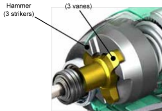
Mechanism of the Triple Hammer
