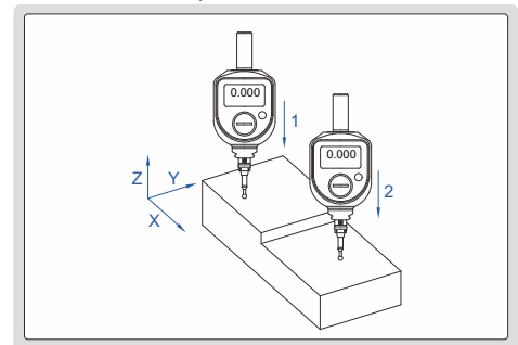
depth measurement
