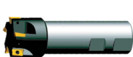
APKT 160408 Inserts
