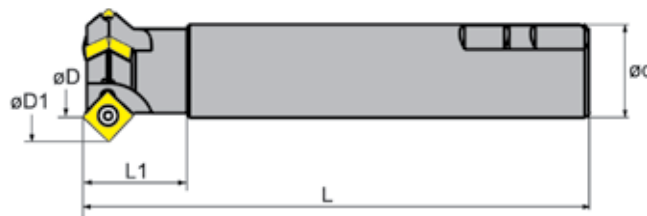
CMA01 Chamfer Cutters Lead Angle 45° - Weldon Shank
